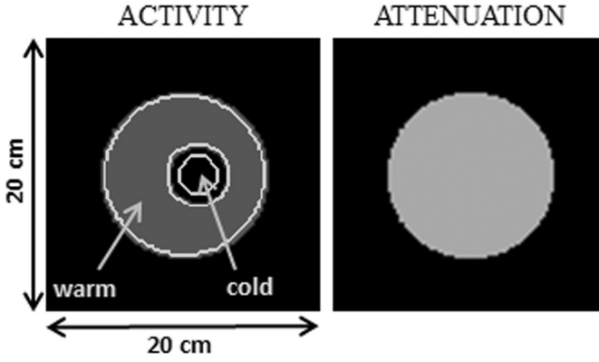
Fig. 3. Phantom 2. The phantom consists of a warm and cold region. The activity and attenuation are shown. The phantom is assumed to have uniform water attenuation.
