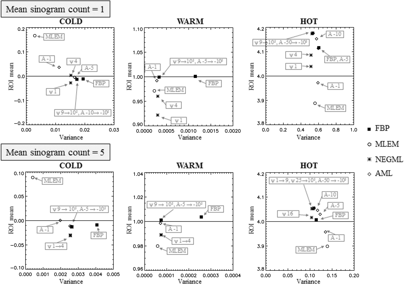
Fig. 8. Phantom 1. Mean with respect to variance in the cold regions, warm region and hot region for different values of \psi and A . The chosen frame duration correspond to on average 1 and 5 counts per sinogram pixel. The solid line represent the true value for each region. Ordinary Poisson with randoms smoothing.
