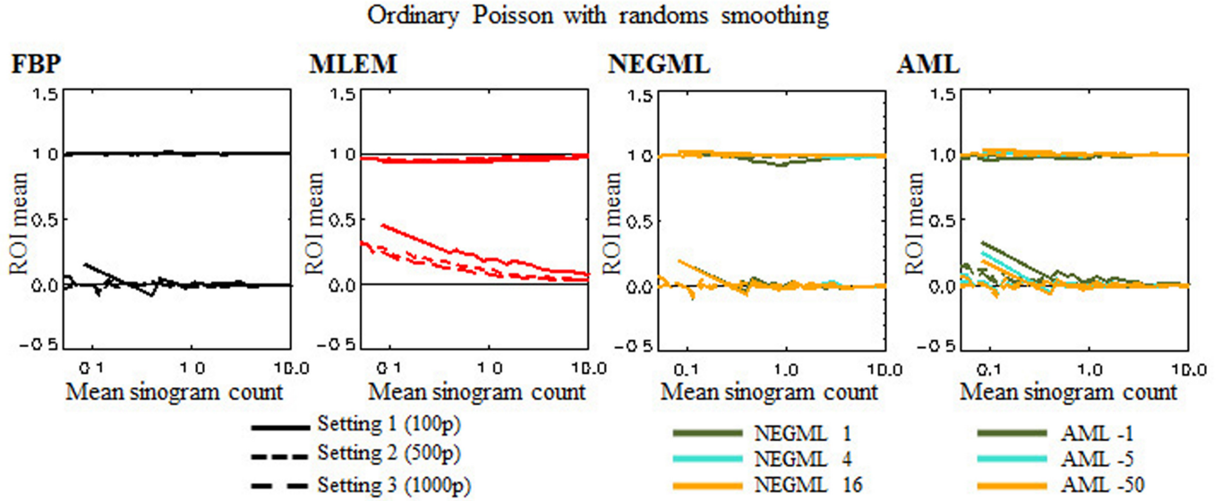
Fig. 10. Phantom 2. ROI mean in the cold and warm region for three setting. Setting 1: 100 projections angles (solid line), setting 2: 500 projection angles (small dashes), setting 3: 1000 projection angles (long dashes).
