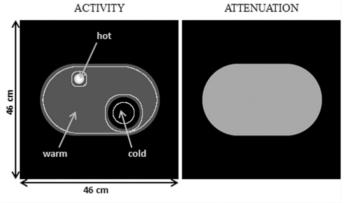
Fig. 2. Phantom 1. The phantom has a cold, warm and hot region. The activity for the main experiment was 0 for the cold region, 1 for the warm region and 4 for the hot region. In a second setting, the phantom's activity was multiplied by three. The phantom is assumed to have uniform water attenuation.
