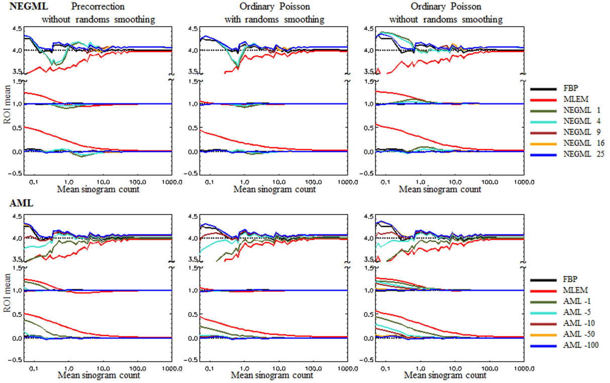
Fig. 4. Phantom 1. Evaluation of the ROI Mean for different frame durations. The frame duration is represented by the mean number of counts per sinogram pixel in the frame. Three different ways for randoms handling are shown. The upper row gives the results for NEGML, the lower row shows the results for AML.
