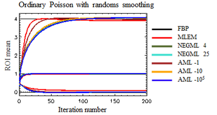
Fig. 9. Phantom 1. Convergence of MLEM, NEGML (with \psi = \{4, 25\} ) and AML (with A = \{-1, -10, -10^5\} ). The value for FBP is given as a reference
