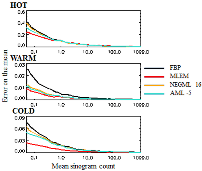
Fig. 5. Phantom 1. The standard error on the mean for the Ordinary Poisson method with randoms smoothing (figure 4) for FBP, MLEM, NEGML 16 and AML -5 in the cold, warm and hot region of phantom 1.
