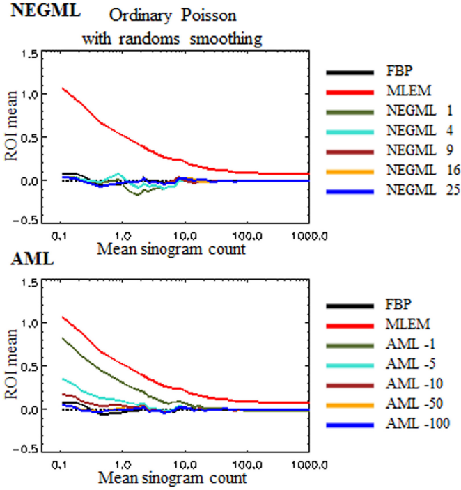
Fig. 6. Phantom 1 with threefold increased activity. Evaluation of the ROI Mean for the cold regions for different frame durations with ordinary Poisson. The frame duration is represented by the mean number of counts per sinogram pixel in the frame. The upper row gives the results for NEGML, the lower row shows the results for AML.
