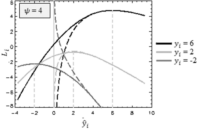
Fig. 1. The standard likelihood function (dashed lines) is drawn for y_i = 6 (black), y_i = 2 (light grey) and y_i = -2 (dark grey). The corresponding modified likelihood functions with \psi = 4 , as proposed in Eq. (6), are drawn as solid lines.
